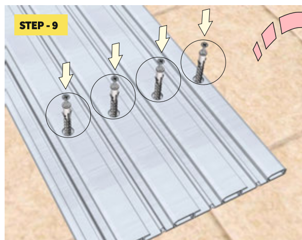
STEP - 9 Insert the raw-plug into a cleaned hole
