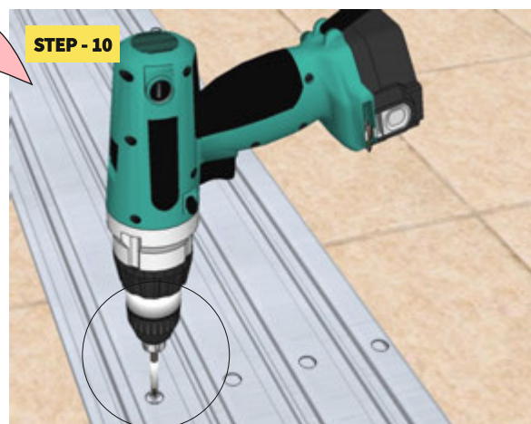
STEP - 10 Slightly hammer in tight the rail to the ground by screws!
