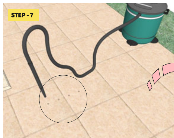
STEP - 7 Don´t forget to clean the dirt from drilling holes under the rails, use vacuum cleaner.
