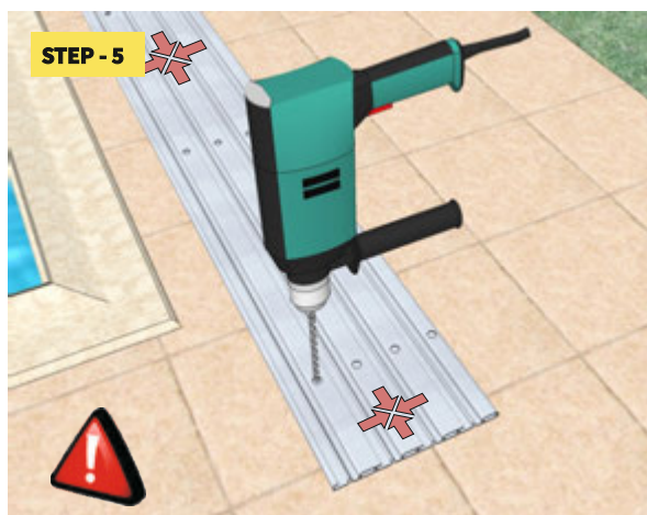
STEP - 5 Drilling through this one complet rail according the number of predrilling holes in rail. During drilling avoid the shifting of rail!
